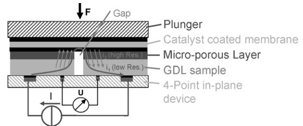
Fig. 11. Measurement setup for determination of sublayer resistance in combination with sublayer-catalyst layer contact resistance over compression. A small gap in the GDL sample is used to force current through the GDL-catalyst layer interface.
